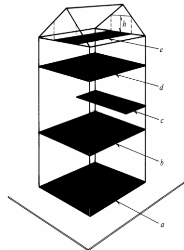
Floor Area Floor Area = a + b + c + d + e (include e only if h \geq 7'10'' )
